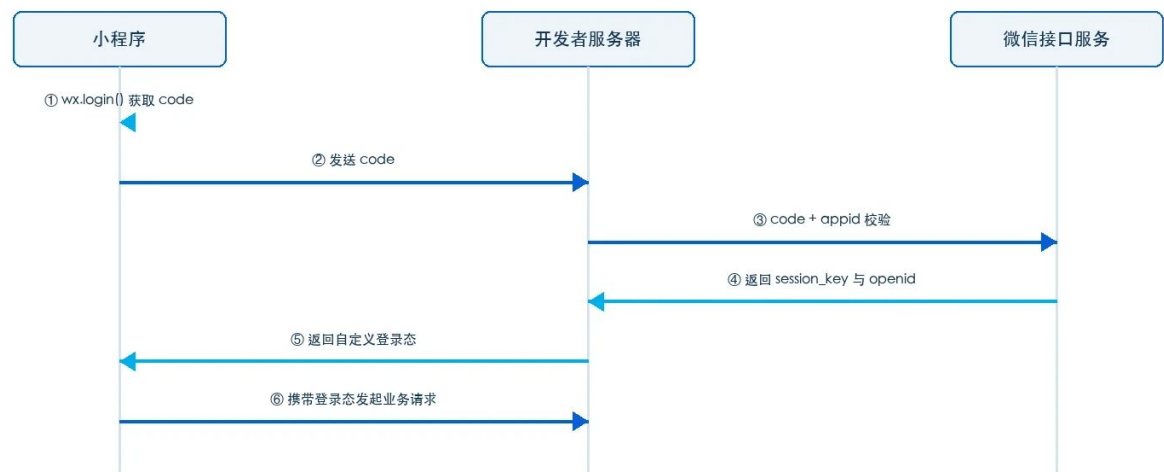
A six-step interactive process between the applet, the developer server and the micro-intelligence interface service to complete authorized login.
