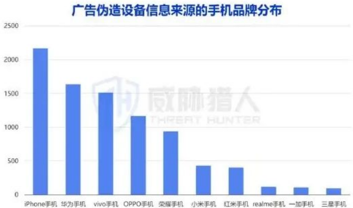
Analysis of brand advertising fraud scenarios (Chart 2)
